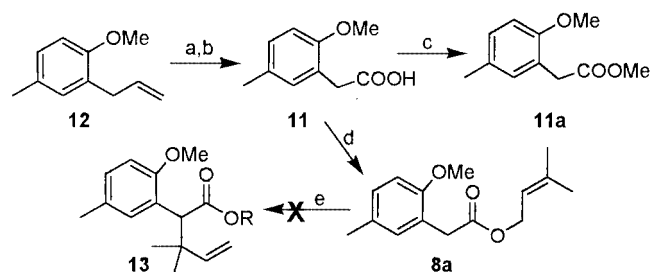
Scheme 2. Reagents, conditions and yields: (a) O_3/O_2 , CH_2Cl_2/MeOH (4:1); Me_2S , 4 h; 86%; (b) Jones reagent, Me_2CO , 0 °C \rightarrow room temp., 2 h, 88%; (c) MeOH , H_2SO_4 , reflux, 8 h, 90%; (d) Me_2C=CHCH_2OH , DCC, DMAP, CH_2Cl_2 , 6 h, room temp., 88%; (e) LDA, TBDMSCl; \Delta
