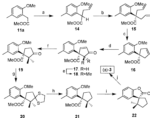
Scheme 3. Reagents, conditions and yields: (a) LDA, THF, -70 °C; CH_2=CHCH_2Br , \rightarrow room temp., 4 h; 92%; (b) LDA, THF, HMPT, -70 °C; CH_2=CHCH_2Br , \rightarrow room temp., 8 h; 86%; (c) 5 mol% [PhCH= RuCl_2(PCy_3)_2] , CH_2Cl_2 , room temp., 4 h, 95%; (d) PDC, py, 100 °C, 8 h, 65%; (e) NaH, DME, MeI, room temp., 12 h, 71%; (f) H_2 (1 atm), 5% Pd/C, EtOH, 2 h, 90%; (g) (CH_3SH)_2 , BF_3 \cdot Et_2O , C_6H_6 , 0 °C \rightarrow room temp., 4 h, 83%; (h) Raney Ni, EtOH, reflux, 3 h, 85%; (i) BBr_3 , CH_2Cl_2 , -40 °C \rightarrow room temp., 4 h, 65%; (j) ref. [4]
